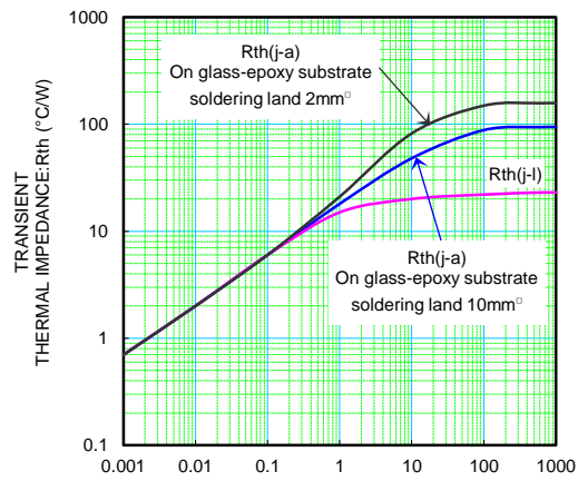
Rth-t CHARACTERISTICS
